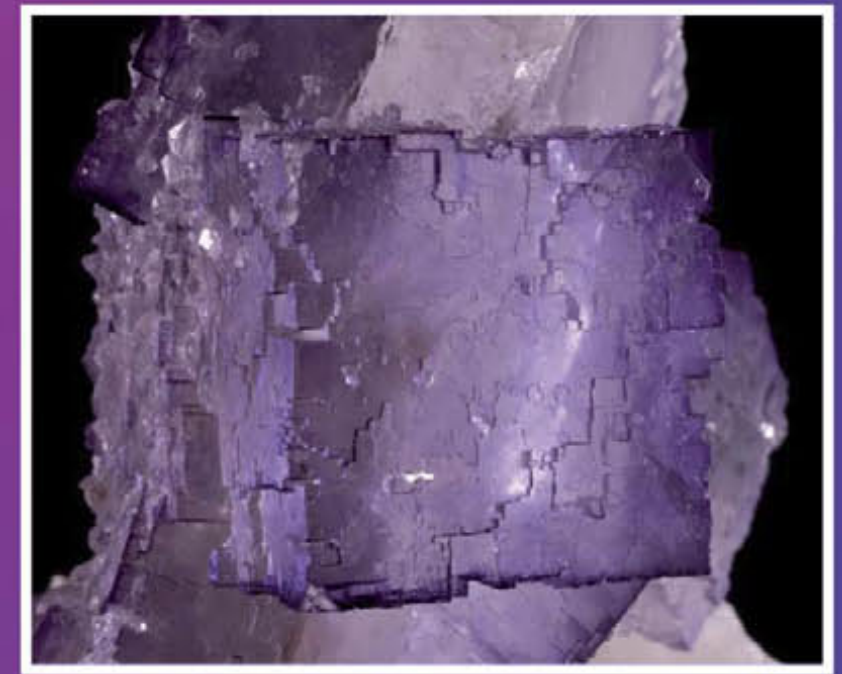
Details of the growth forms of fluorite crystals. © Grenoble Natural History Museum
